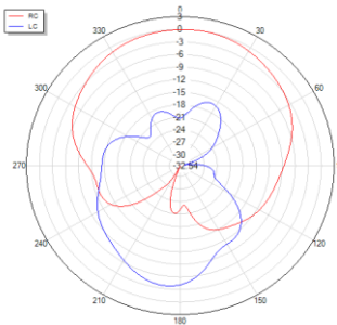
Phi=90 freq=1176MHz
