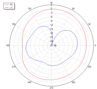
Theta=90 freq=1207MHz
