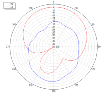
Phi=0 freq=1207MHz
