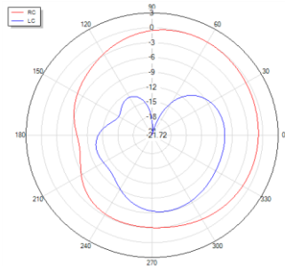
Theta=90 freq=1176MHz
