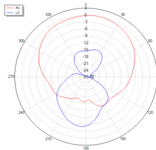
Phi=90 freq=1207MHz
