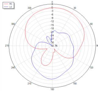
Phi=0 freq=1176MHz
