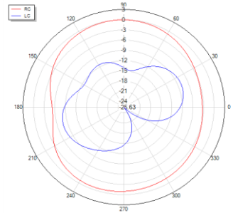
Theta=90 freq=1248MHz
