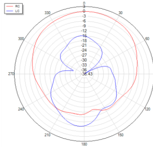
Phi=90 freq=1248MHz
