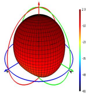
Phi=90 freq=1248MHz
