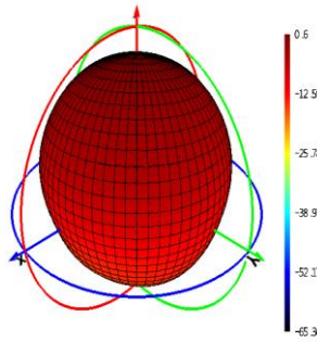
Phi=90 freq=1176MHz
