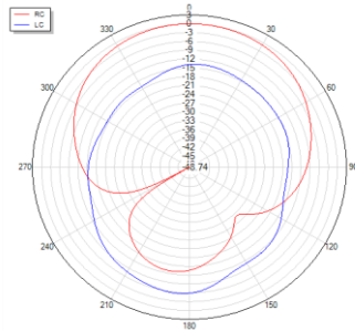
Phi=0 freq=1227MHz
