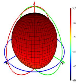
Phi=90 freq=1207MHz
