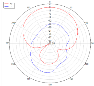
Phi=0 freq=1248MHz
