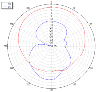
Phi=90 freq=1227MHz
