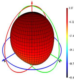
Phi=90 freq=1227MHz
