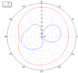
Theta=90 freq=1227MHz
